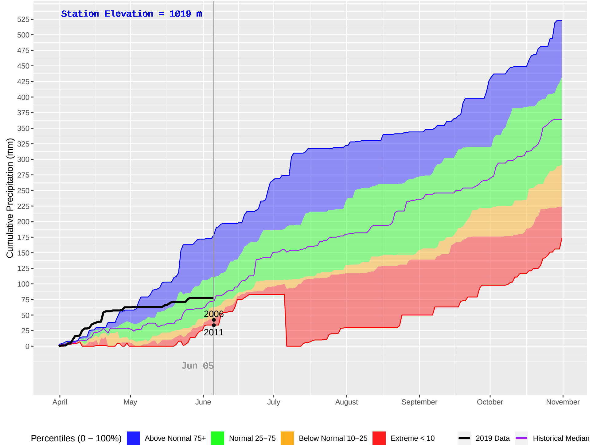
POWDER CREEK (380) : Historical (2001–2018), Current (2019) Daily Cumulative Precipitation
