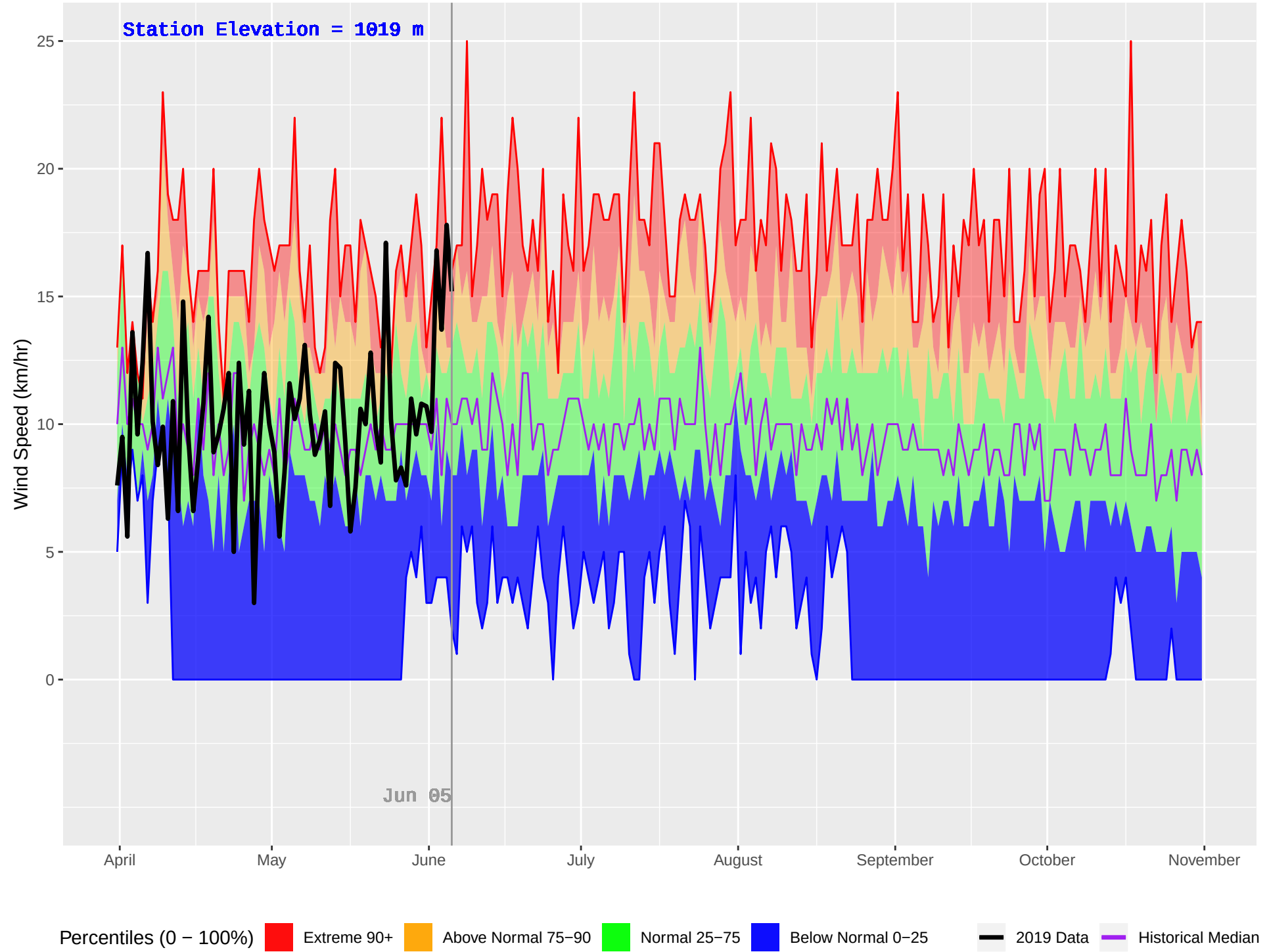
POWDER CREEK (380) : Historical (2001–2018) and Current (2019) Daily Wind Speed
