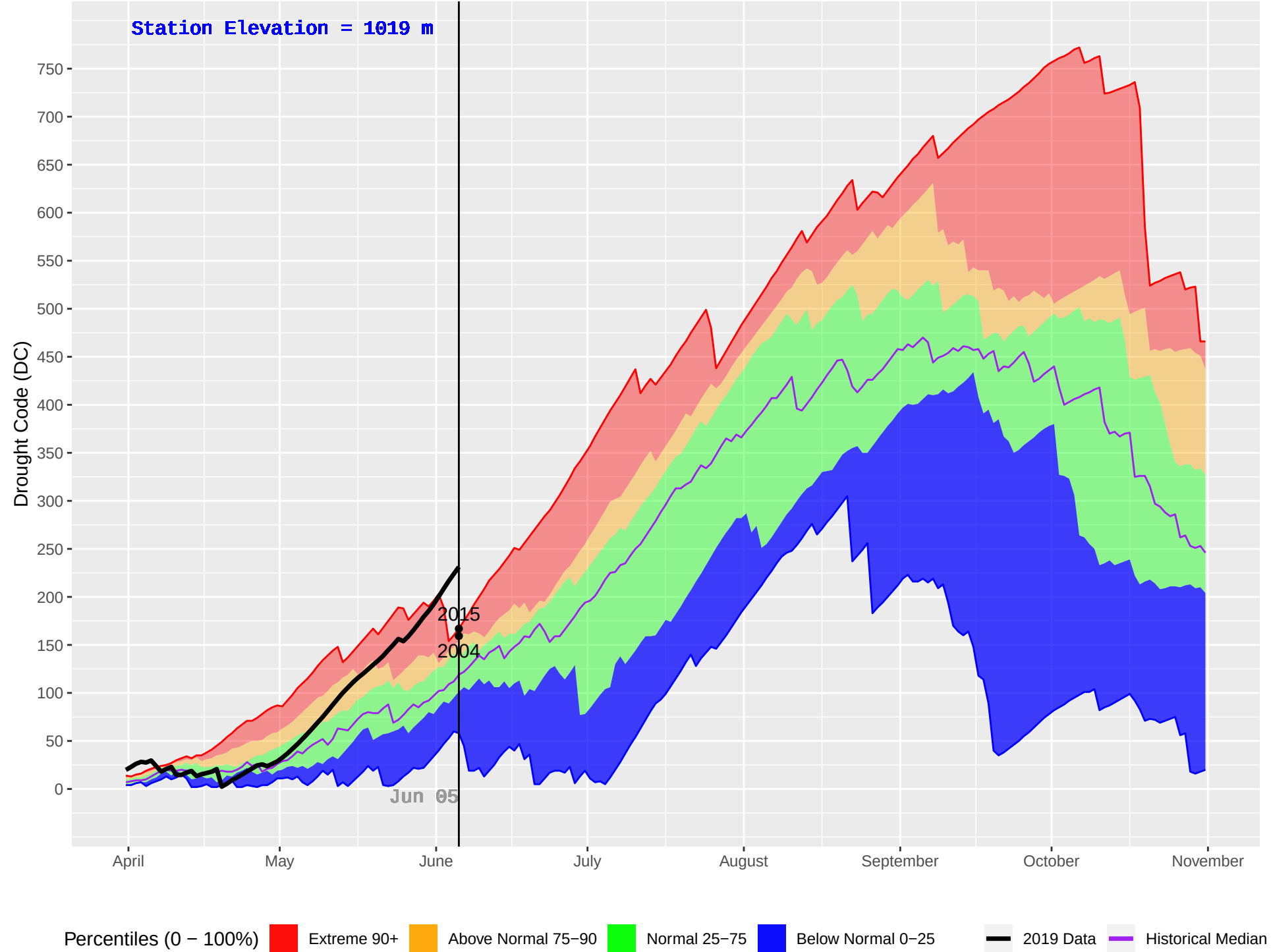
POWDER CREEK (380) : Historical (2001–2018) and Current (2019) Daily Drought Code (DC)
