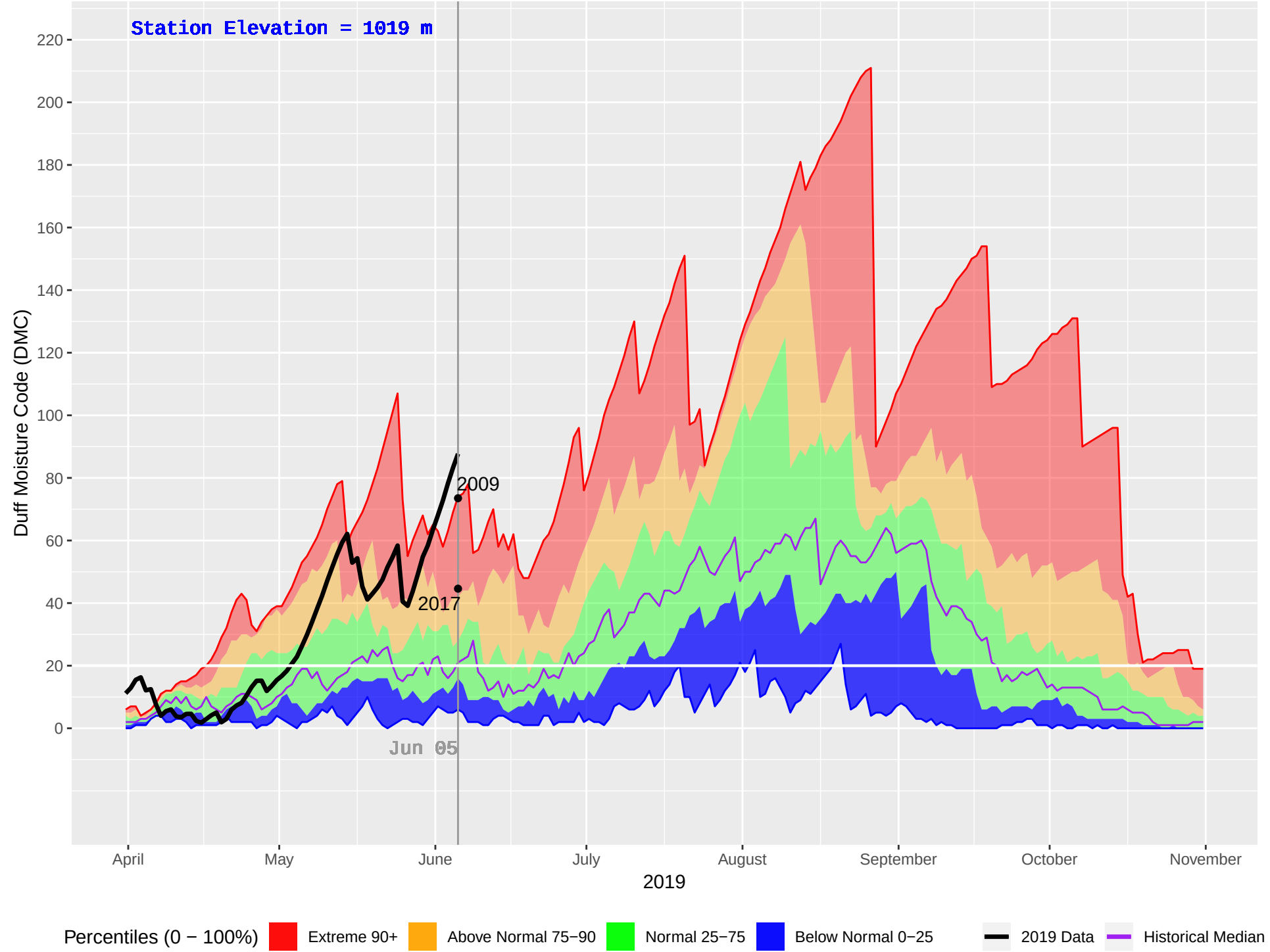
POWDER CREEK (380) : Historical (2001–2018), Current (2019) Daily Duff Moisture Code (DMC)
