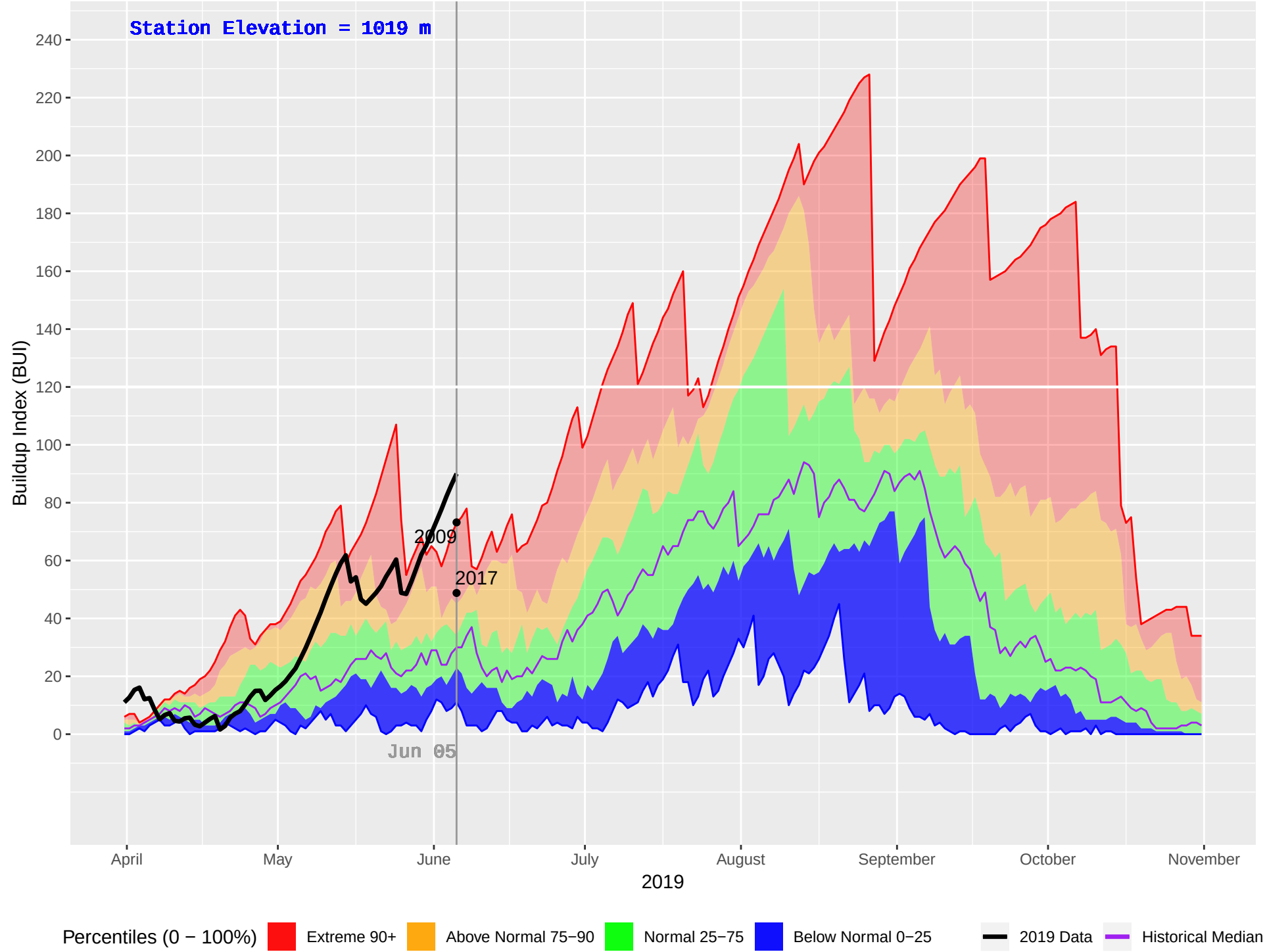
POWDER CREEK (380) : Historical (2001–2018), Current (2019) Daily Buildup Index (BUI)
