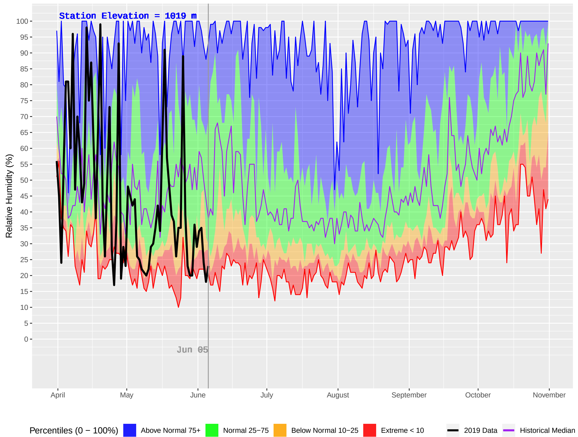
POWDER CREEK (380) : Historical (2001–2018) and Current (2019) Daily Relative Humidity
