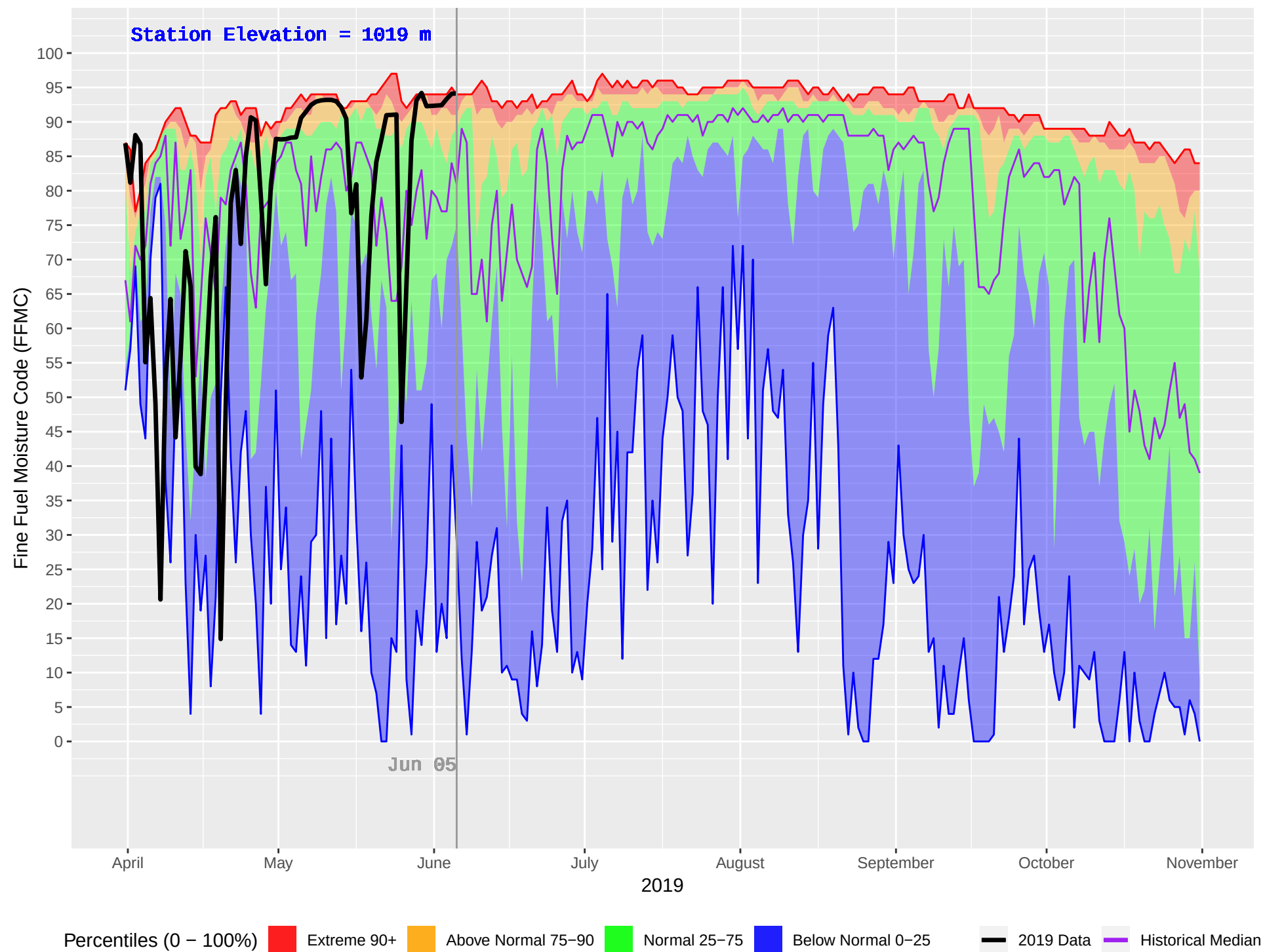
POWDER CREEK (380) : Historical (2001–2018) and Current (2019) Daily Fine Fuel Moisture Code (FFMC)
